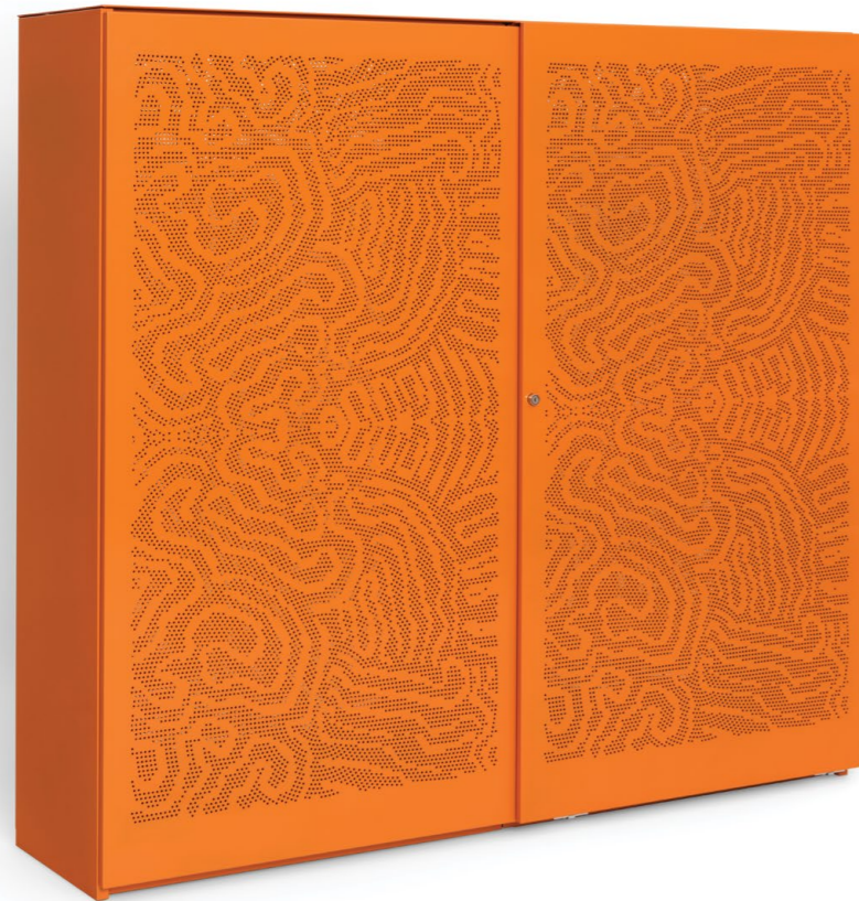
“Yuurra-gi” signature perforation design inspired by notions of movement, collaboration with Lucy Simpson, exclusive to Planex W 1800 H 1675 (includes 3mm top) D 500
